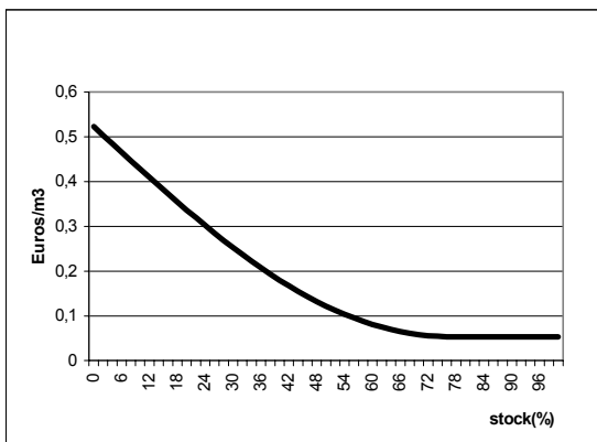
Fig.2: Correspondence \lambda = \Gamma(S) in EV
