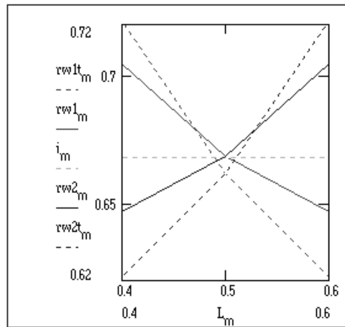
Fig.6 - Bilateral protection
