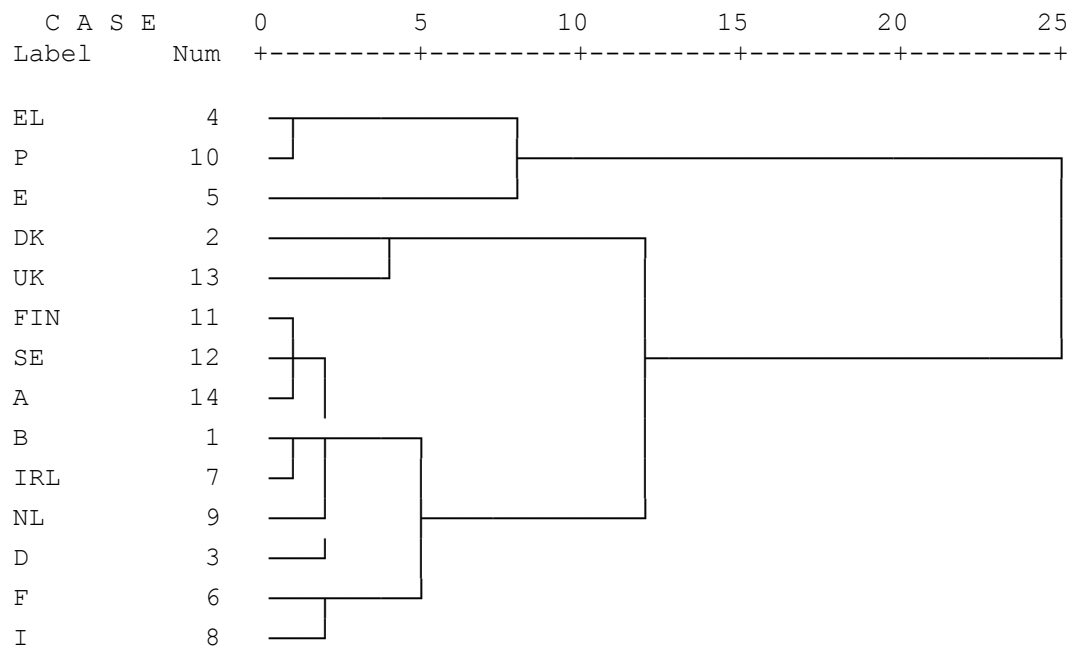
Figure 1d: Dendrogram, Median Linkage, Quadratic Euclidian Distance
