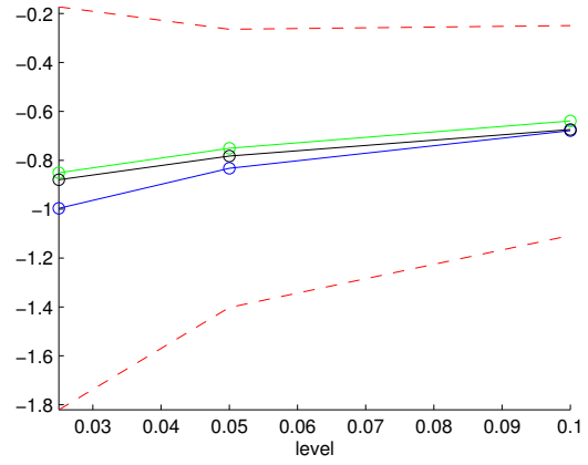
(b) lagged realized volatility
