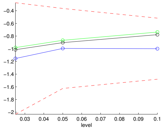
(c) lagged week average realized volatility
