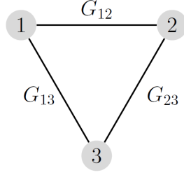
3 4 Figure 1. A network game.
