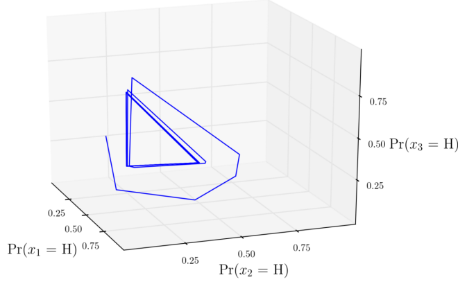
Figure 4. Fictitious play need not converge in a network of conflicts.
