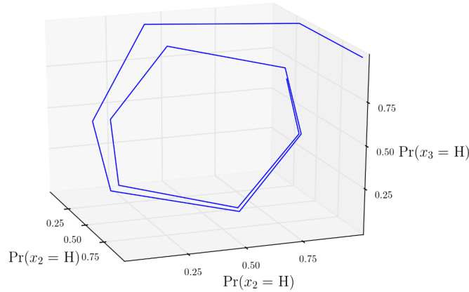
5 6 Figure 6. A network of weighted potential games need not possess the CTFP property.
