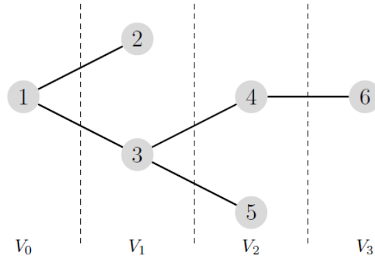
13 14 Figure 3. Partitioning the set of nodes in an acyclic network.
