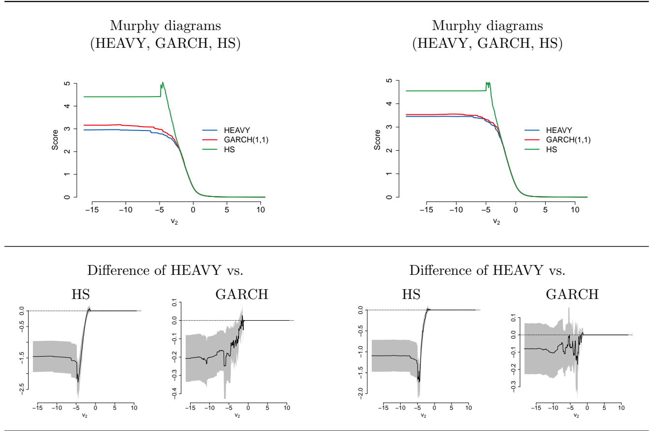
Figure 2: Murphy diagrams for empirical forecasts. Top panels: Smaller scores are better. Bottom panels: Negative difference means that HEAVY outperforms its competitor. Confidence intervals are pointwise at 95% level.
