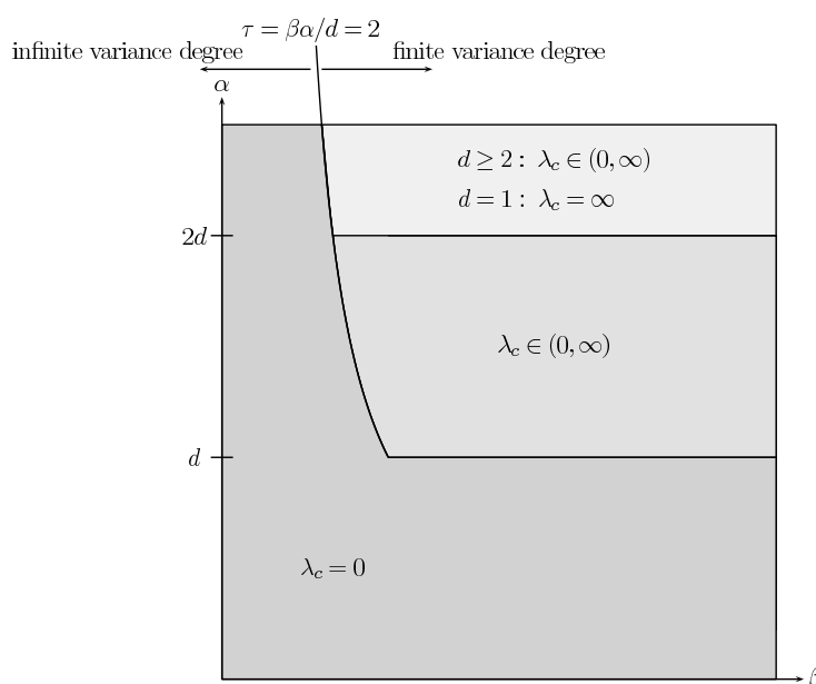
Figure 1. phase transition picture for d \geq 1 .
