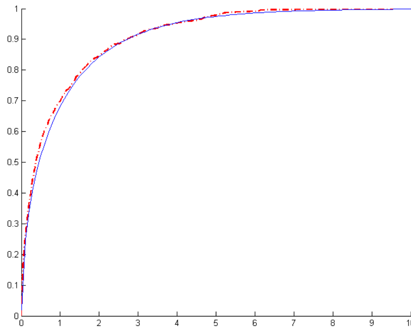
Figure 2. CDF plot for empirical distribution with a known break.
