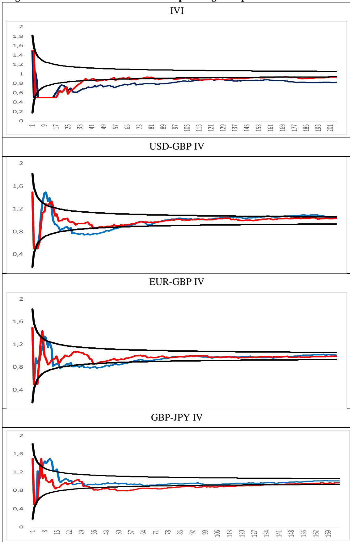
Figure 3: Estimates of d for each subsample using semi-parametric methods
