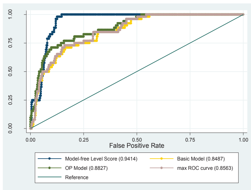
Figure D-1: ROC curves of the model-free level score and model based approaches - qualitative crises dataset
