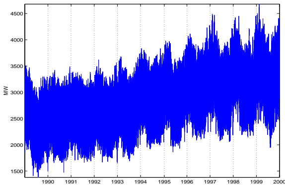
Fig. 1. Hourly loads from January 1, 1990 to December 31, 2000.
