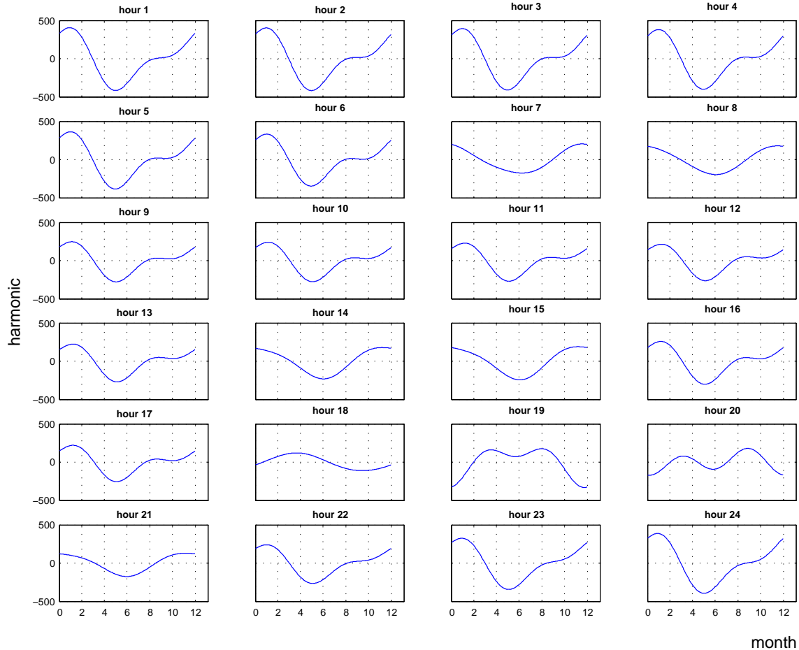
Fig. 3. Estimated harmonic shape for each hour.
