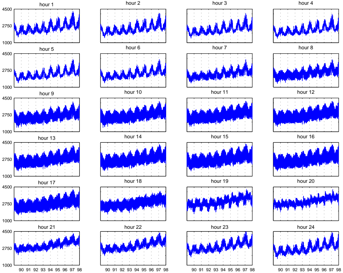
Fig. 2. Load of each hour from January 1, 1990 to December 31, 1998.
