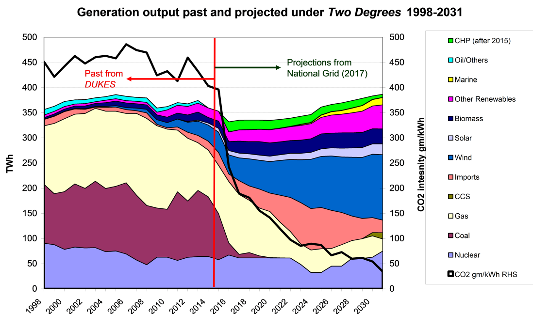
Figure 3: Generation by fuel. Sources: DUKES , National Grid (2017)
