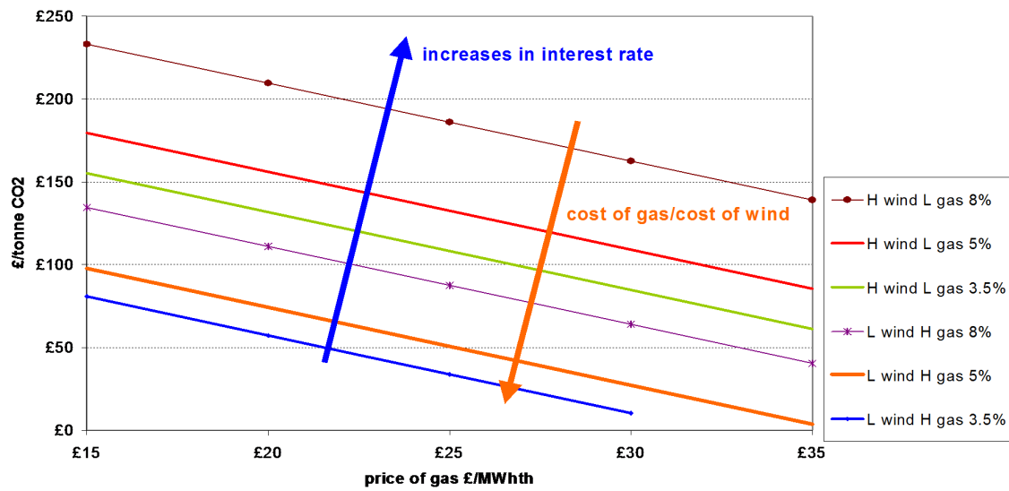
Figure 2: Break-even CO 2 prices vs. the gas price
