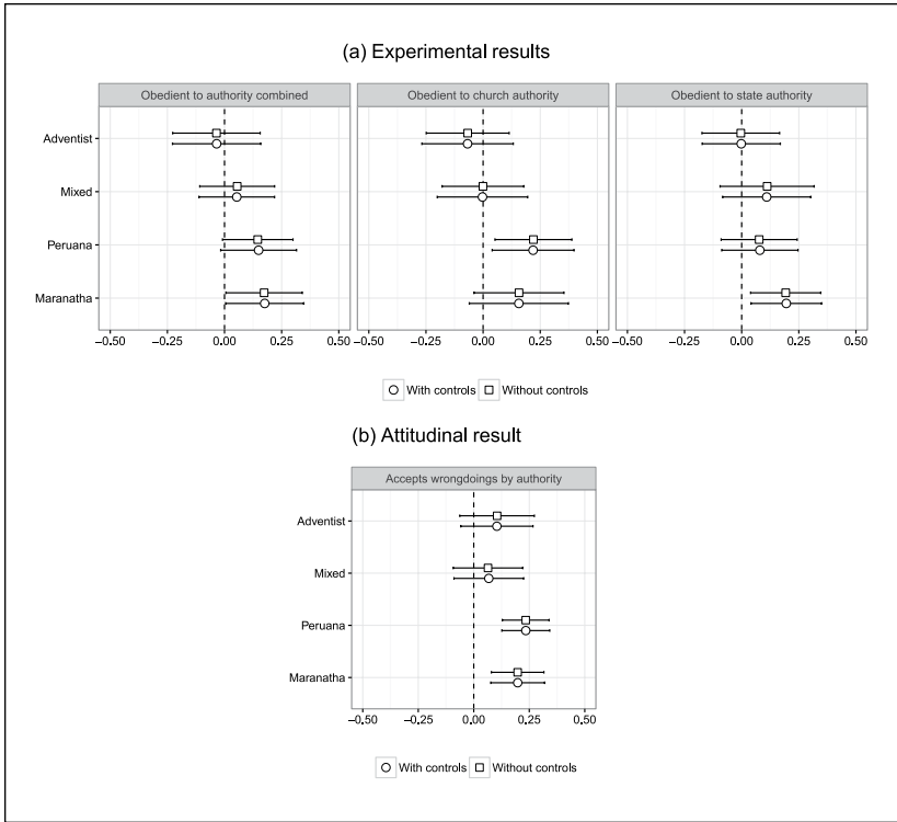
Figure 3. Obedience results.
