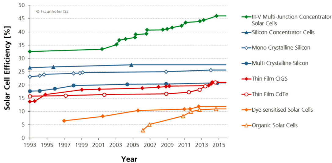
Figure 2: Development of Laboratory Solar Cell Efficiencies
