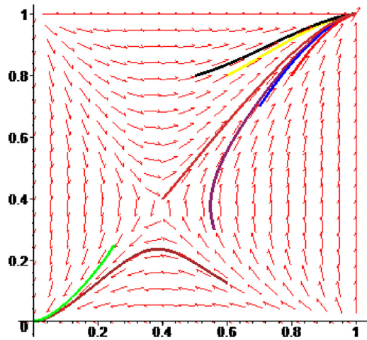
Fig. 1. Phase diagram for case I.
