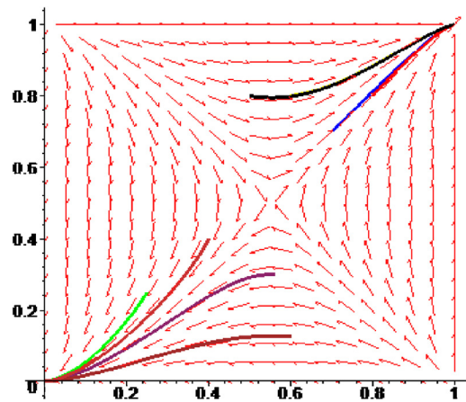
Fig. 2. Phase diagram for case II.
