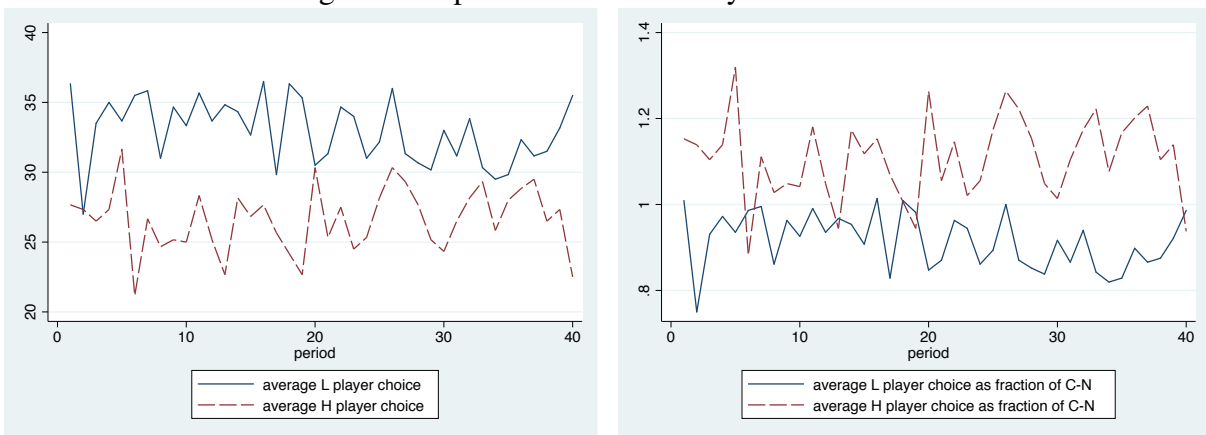
Figure 4: Experimental results: asymmetric firms.
