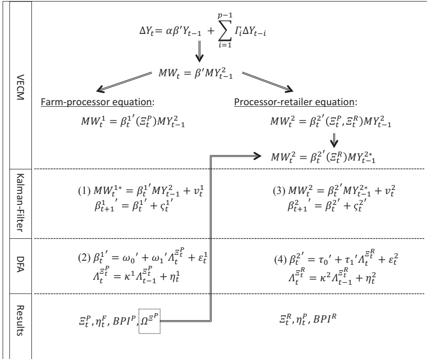
Figure 8: Estimation strategy.
