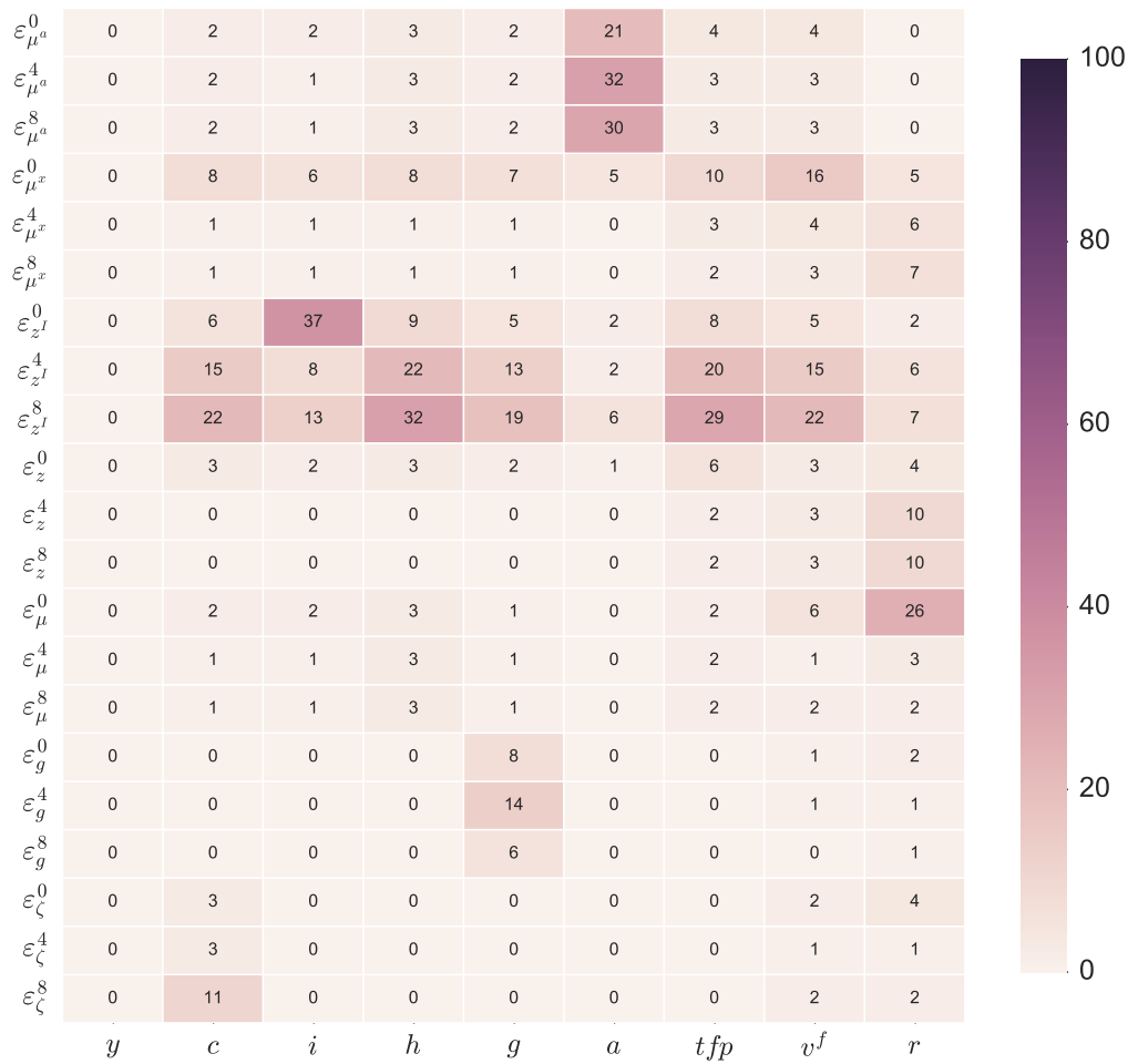
Figure 1: Conditional information gains at MLE of SGU.
