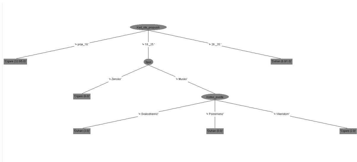
Figure 1 Decision Tree
