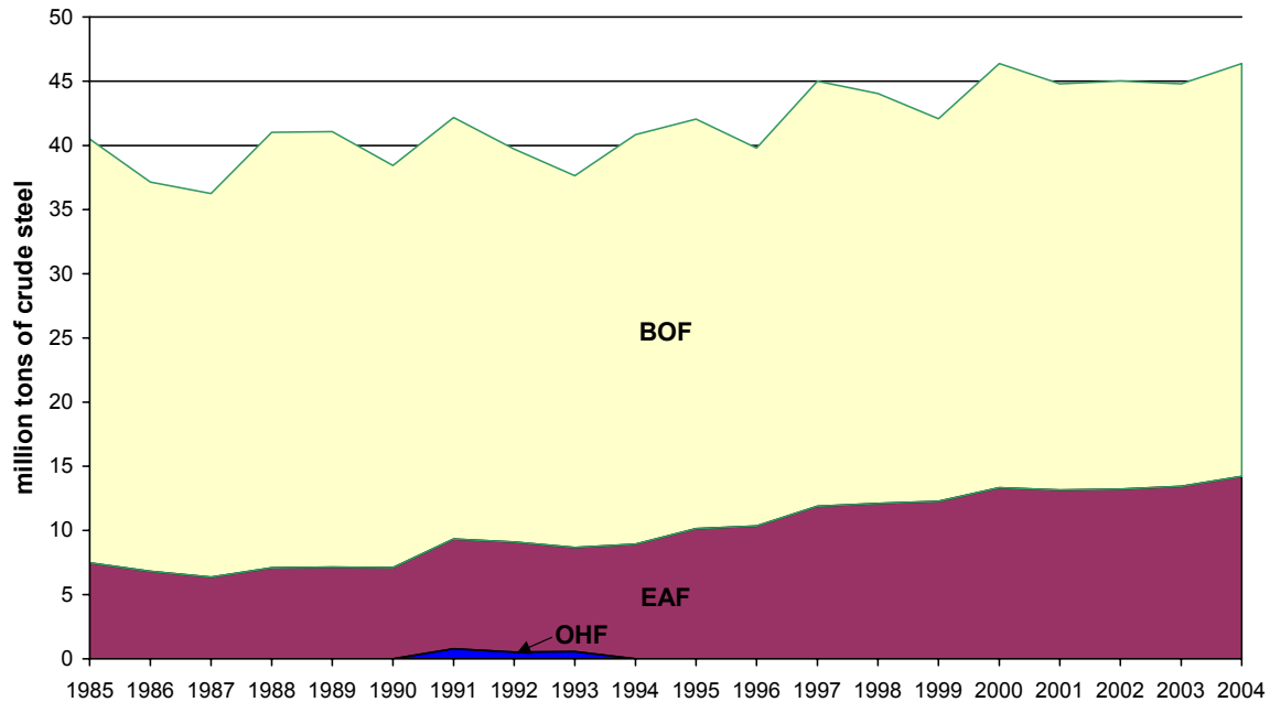
Figure 4 Crude steel production by process type, Germany 1985-2004
