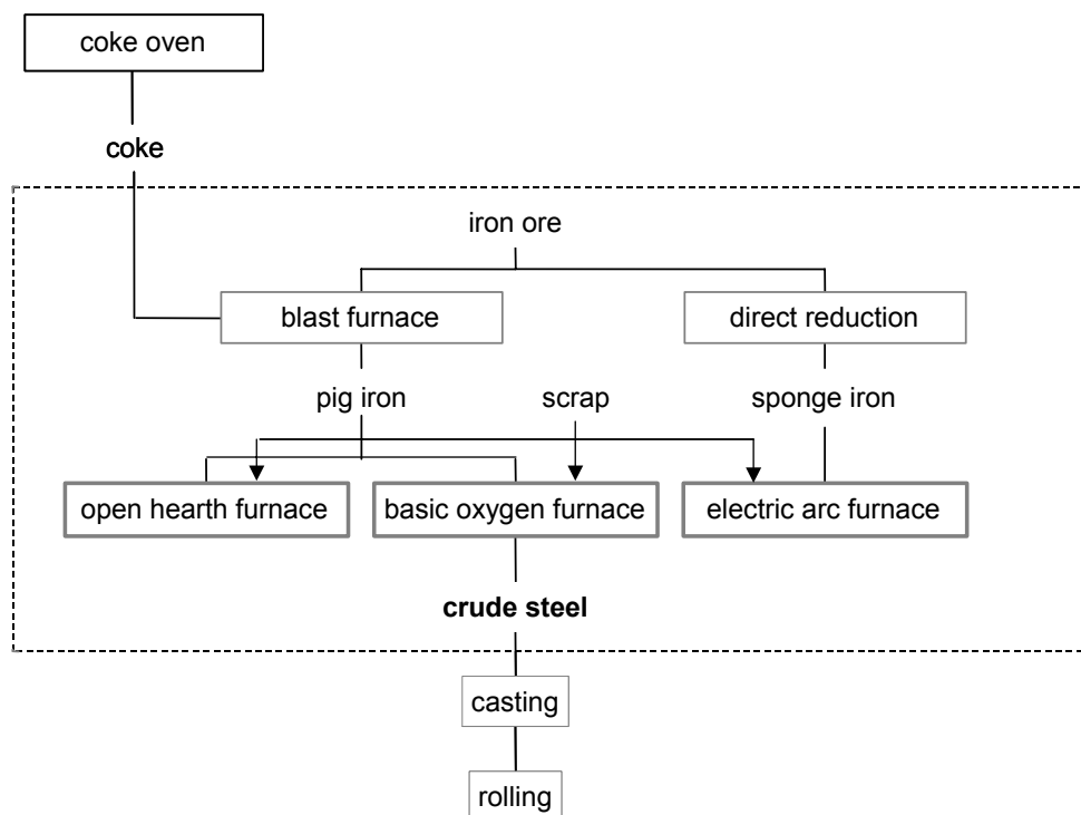
Figure 3 Iron and steel production routes; dotted rectangle indicates system boundary
