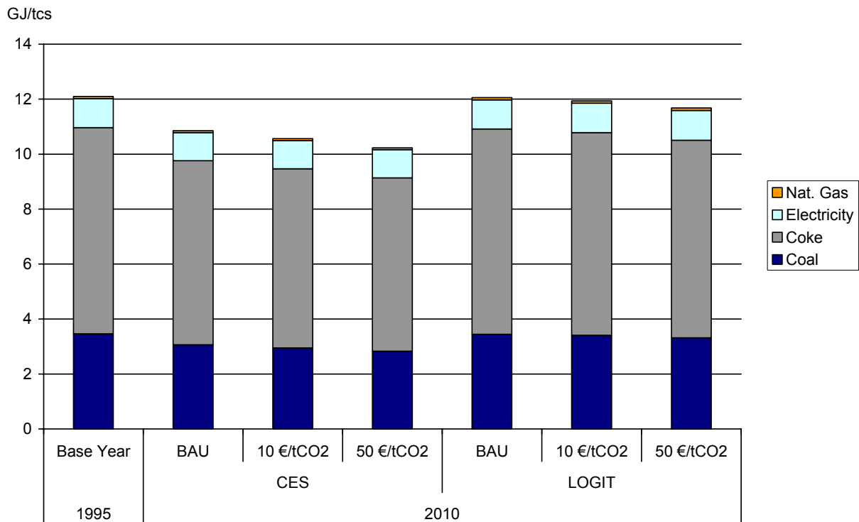
Figure 8 Specific fuel input to iron and steel production, base year and 2010. Units are gigajoules (GJ) per ton of crude steel.
