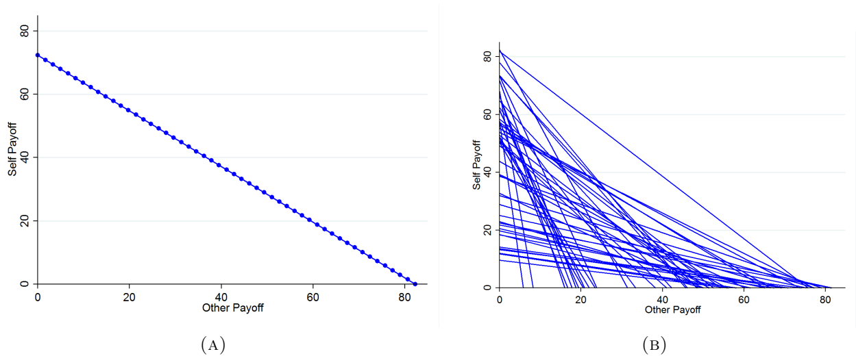
FIGURE E7: GRAPHICAL EXAMPLE OF RANDOMLY GENERATED BUDGET LINES
