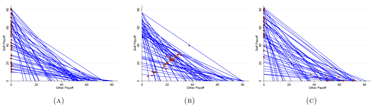
FIGURE E8: GRAPHICAL EXAMPLE OF CHOICES MADE BY SUBJECTS IN THE FKM07 EXPERIMENT
