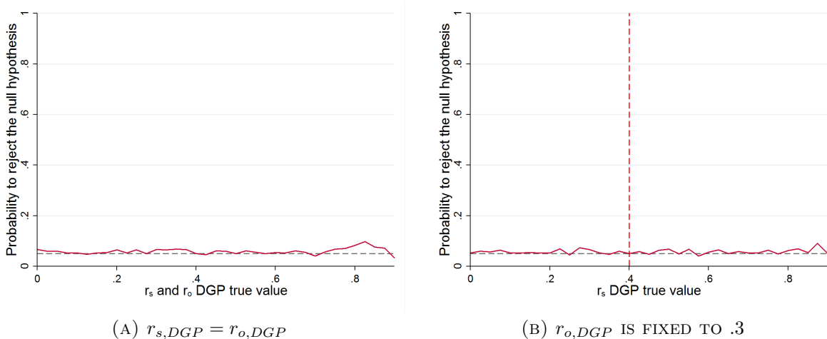
FIGURE B2: POWER CALCULATIONS, TYPE I ERROR
