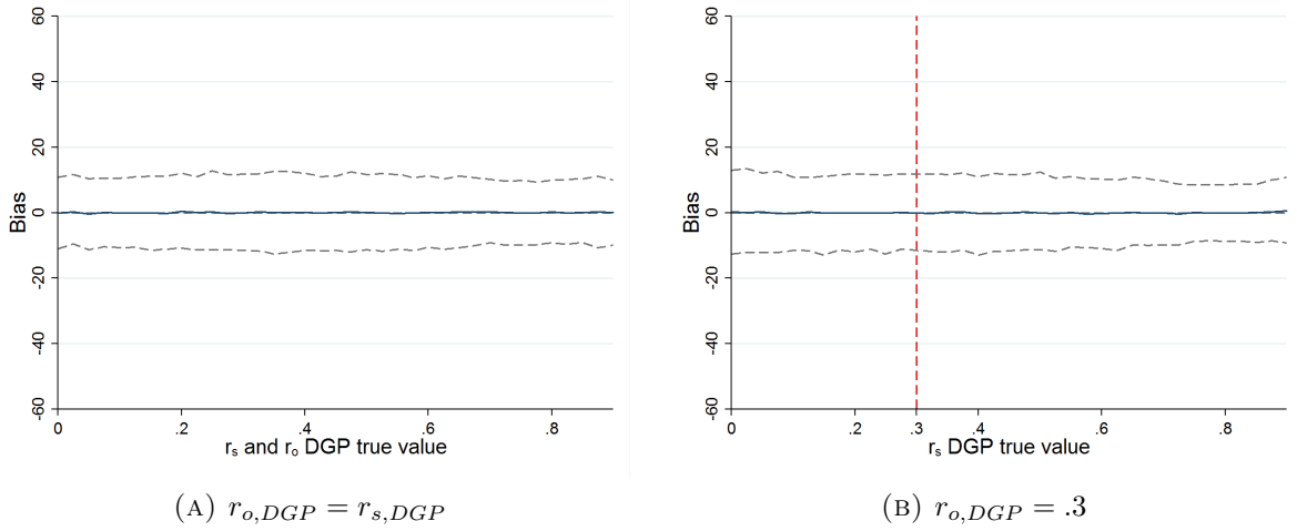
FIGURE B1: BIAS IN ESTIMATED ALTRUISM, \tilde{\alpha}
