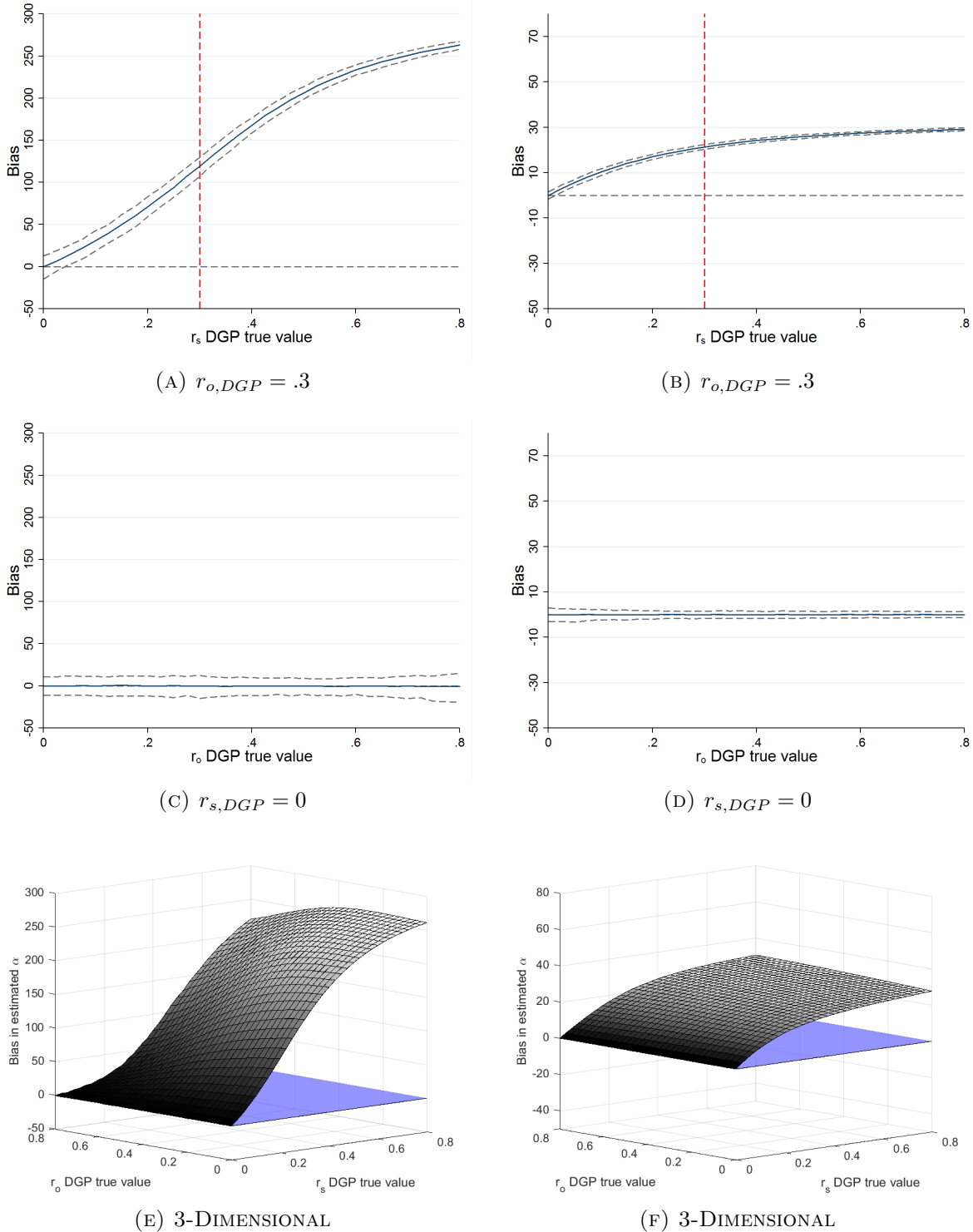
FIGURE F11: BIAS IN ESTIMATED ALTRUISM, \tilde{\alpha} for \alpha_{DGP} = .25 (Left) and \alpha_{DGP} = .75 (Right)
