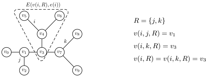
Figure 7: Notions of special nodes in the proof of Theorem 4.2.
