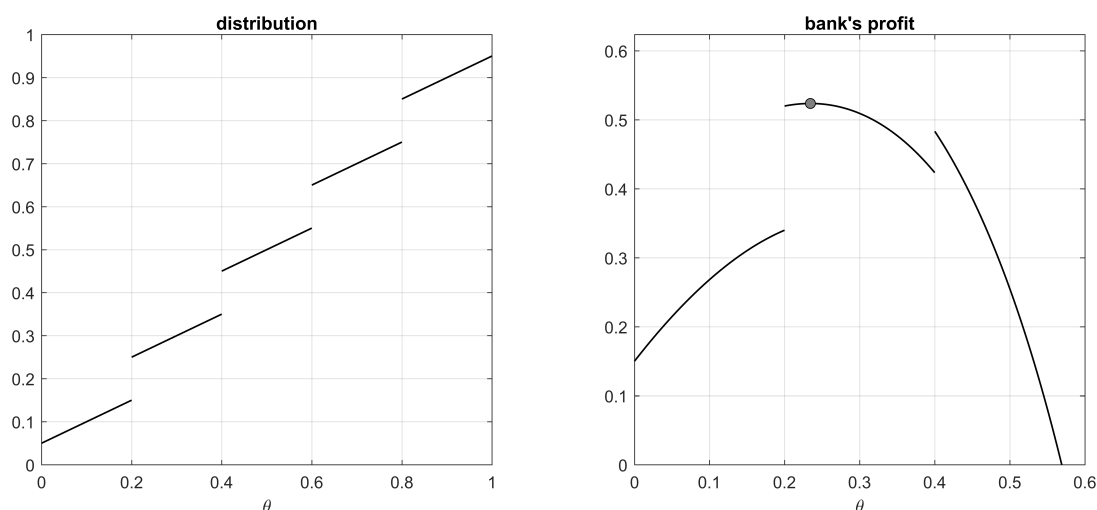
Figure 1: Continuous distribution with a bunch of mass points.
