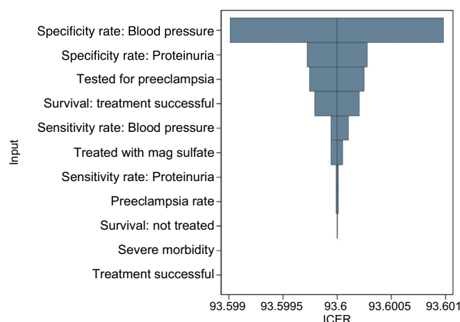
Fig. 1. Tornado diagram: One-way sensitivity analysis of cost-effectiveness of pre-eclampsia intervention to variations in decision tree parameters.
