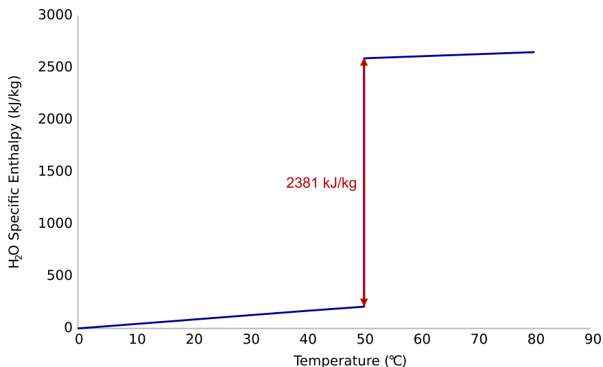
Fig. 6. Energy carrying capacity of water vaporising at 50 °C.
