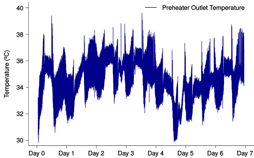
Fig. 8. Preheater outlet temperature over a seven-day period (prior to pressure reduction).
