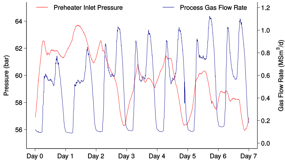
Fig. 7. Preheater inlet pressure and gas flows over a seven-day period.
