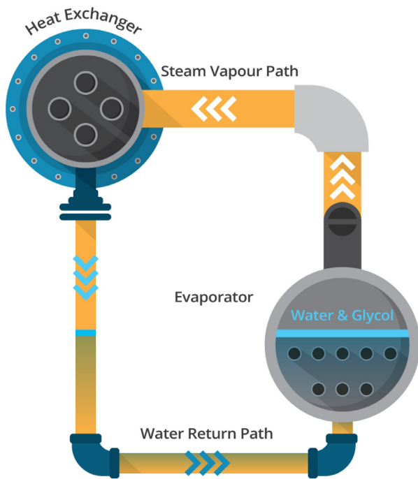
Fig. 5. Configuration of the immersion tube thermosyphon heater (ITTH).
