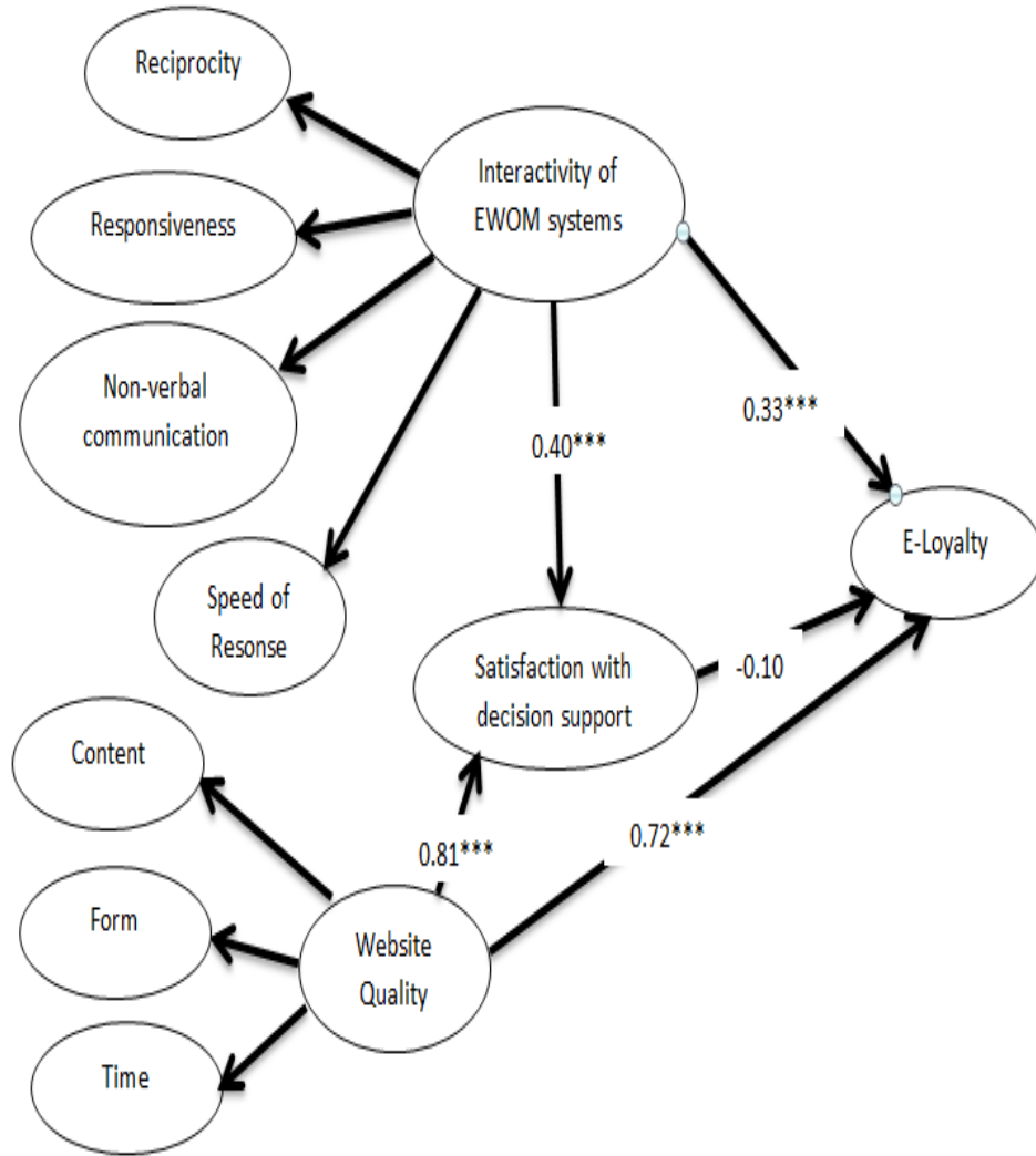
Figure 2: Structural Model with Standardized Coefficients
