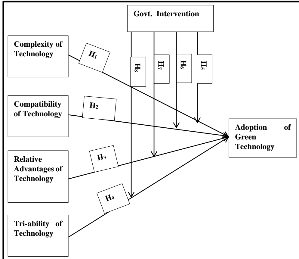
Figure 1: Conceptual Model
