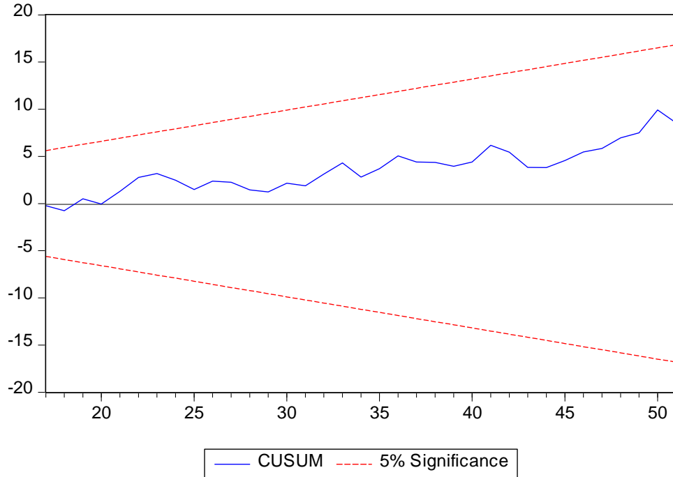
Figure-1: Plot of CUSUM
