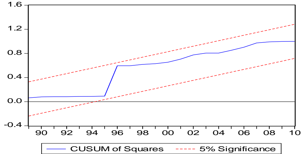
Figure 2: Plot of CUSUMsq
