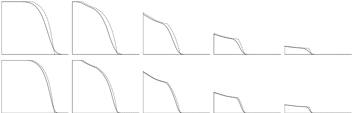
Figure 5: Rows are sample sizes (top is N = 500 , bottom is N = 2000 ). Columns are five values of p (from left to right: p = 0.1, 0.25, 0.5, 0.75, \text{ and } 0.9 ). Dotted lines are the true breakdown frontiers. The solid lines are the Monte Carlo estimates of \mathbb{E}[\widehat{\text{BF}}(c)] . This plot shows the finite sample bias of our breakdown frontier estimator.
