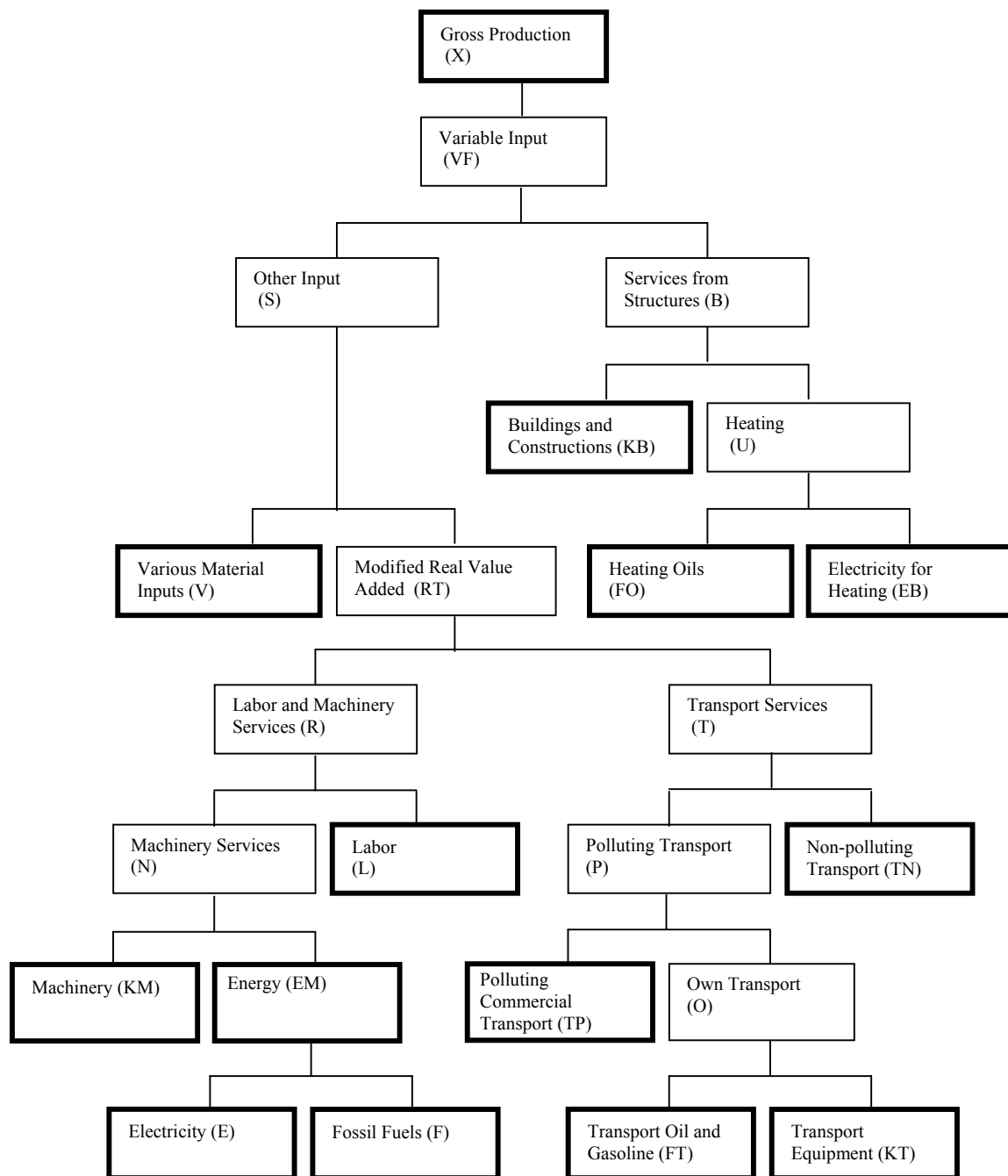
Figure B.1. Production technology
