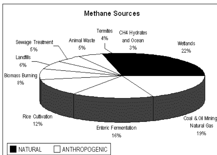
Fig. 1: Sources of Methane Emissions
