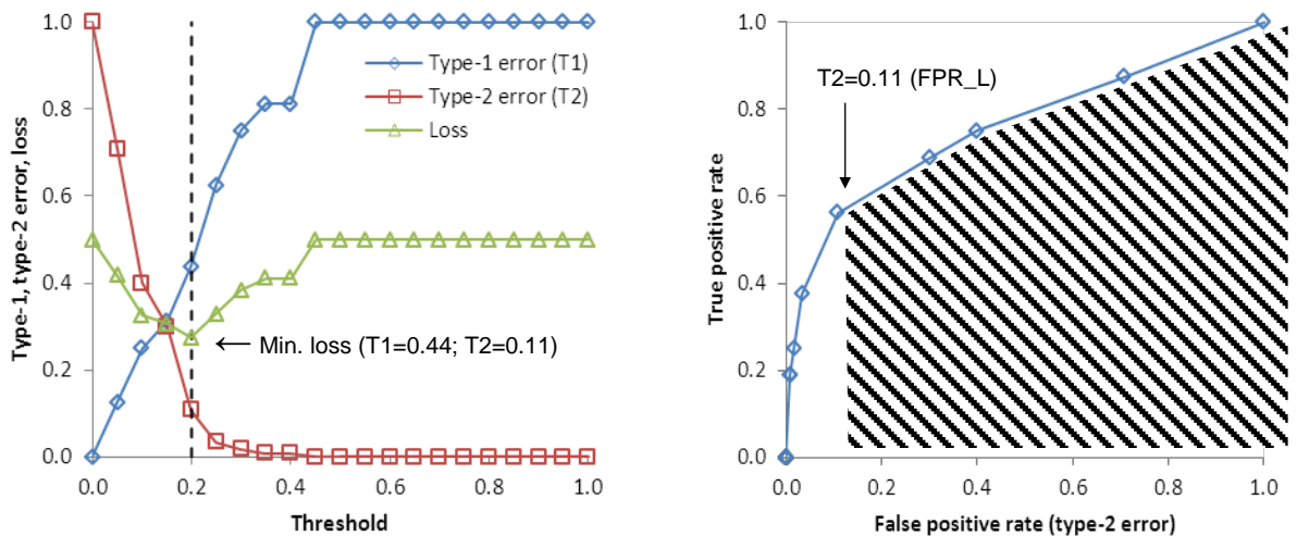
Figure B.1: Restricting the range of false positive rates
