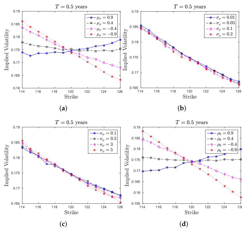
Figure 1. Comparison of implied volatilities for varying each parameter of stochastic correlation processes. (a) Varying \mu_\rho ; (b) Varying \sigma_\rho ; (c) Varying \kappa_\rho ; (d) Varying \rho_0 .
