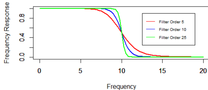
Figure 3. Examples Butterworth Frequency Responses, critical frequency = 10.
