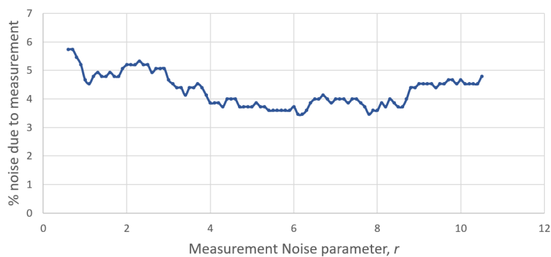
Figure 5. Variation of percentage of signal noise with measurement noise parameter r : organisation FT .
