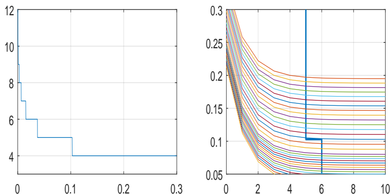
Figure 1. The function M(a) and the running ruin probabilities a_i(s) .
