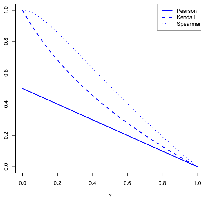
Figure 2. The plot of the Pearson rho, Kendall tau, and Spearman rho measures of correlation for varying values of \gamma \in (0, 1) .
