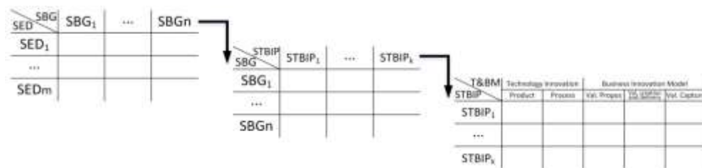
Figure no. 1: Related Matrices Framework (RMF)
