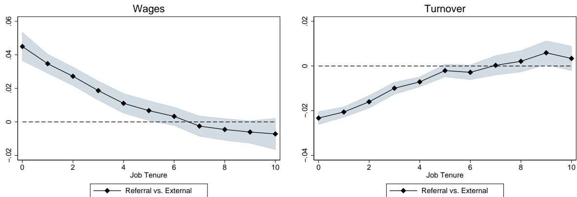
FIGURE 4: CONVERGENCE PROFILES
