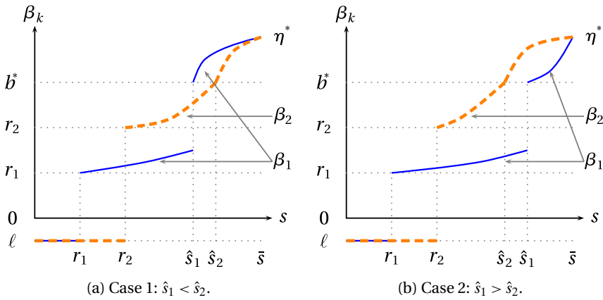
FIGURE 2. Group-symmetric equilibria in an asymmetric first-price auction.
