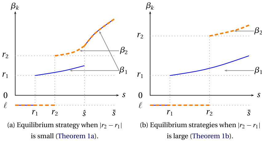
FIGURE 1. Equilibrium strategies in the first-price auction with reserve prices r_1 < r_2 .
