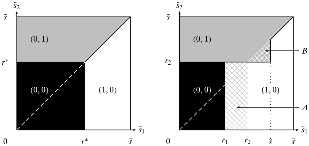
(a) (\psi_1, \psi_2) with a common reserve price r^* .
