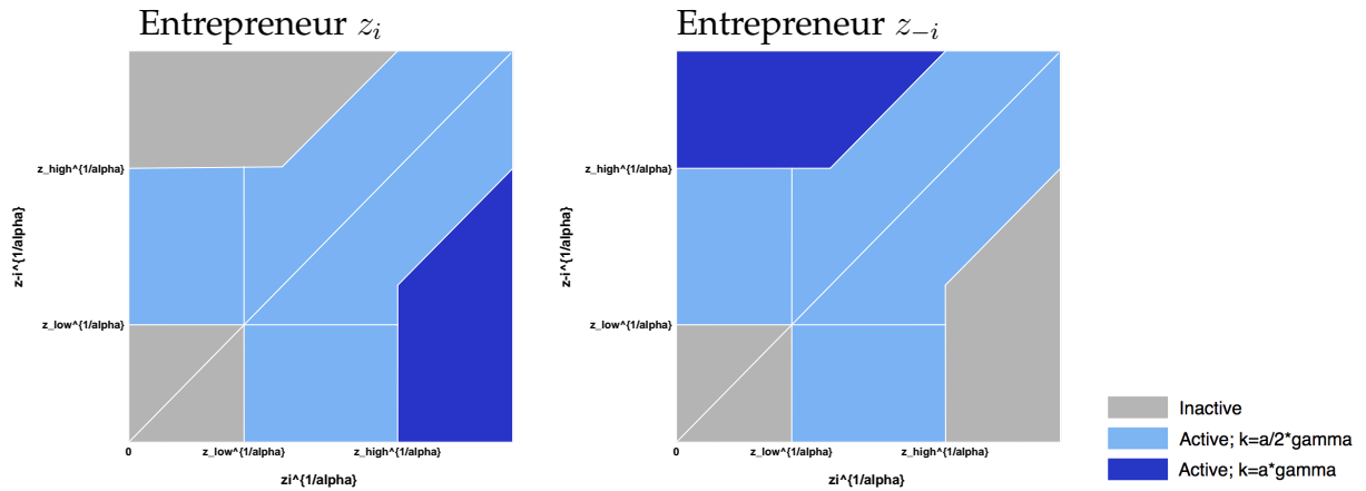
Figure A5: The cut-off rule when \epsilon \in (0, \infty)
