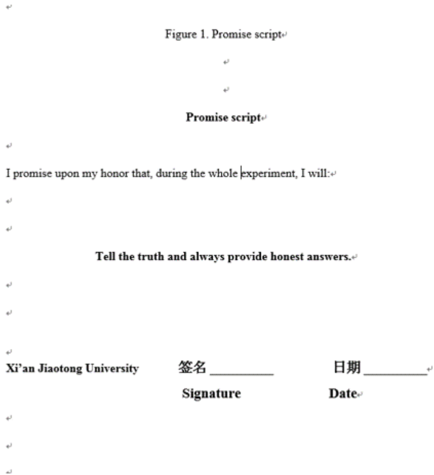
Figure 1: Promise script
