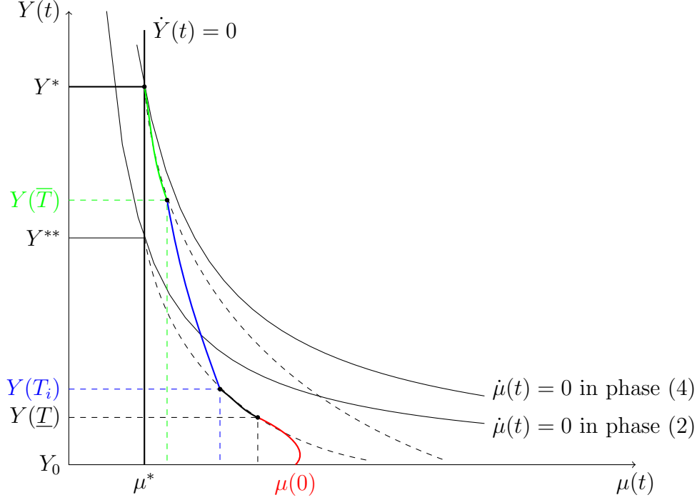
Figure 2: Global phase diagram
