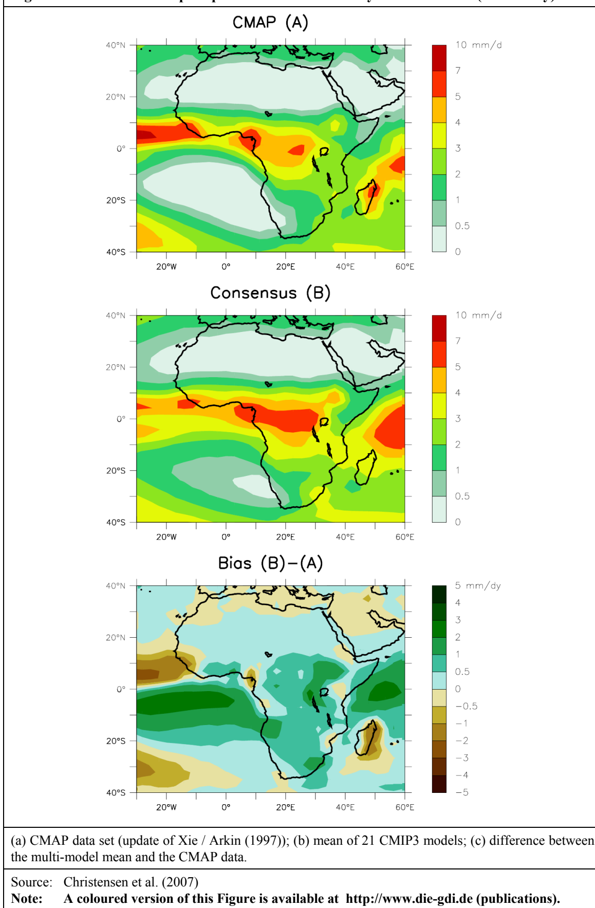
Figure 6: Annual mean precipitation in Africa in the years 1980–1999 (in mm/day)
