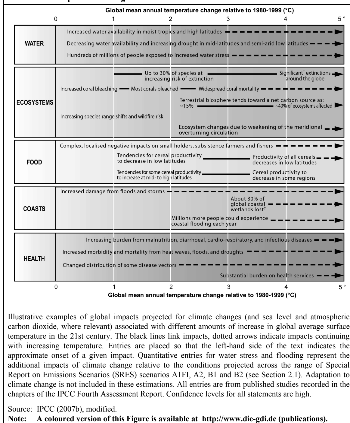
Figure 10: Projected impacts of climate change, ordered by global mean annual temperature change relative to 1980–1999
