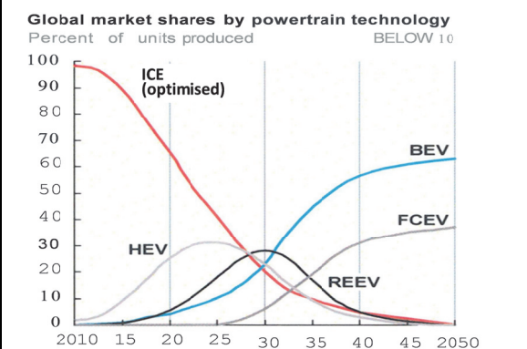
(B) Strict: Fleet emissions below 10 gCO 2 /km by 2050
