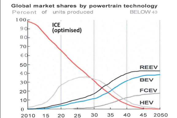
(A) Moderate: Fleet emissions below 40 gCO 2 /km by 2050
