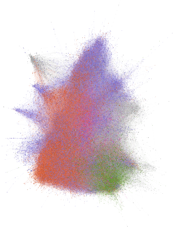
Figure 2: Snapshot of the largest weakly connected component in the Japanese customer-supplier network in 2016. For visual clarity, only firms with sales larger than three billion yen are shown. Nodes colored in purple, orange, and green represent firms operating in the three largest business divisions in the sample. We distinguish purple: retail & wholesale, orange: manufacturing, and green: construction. Firms operating in all remaining sectors are graphically illustrated in gray.
