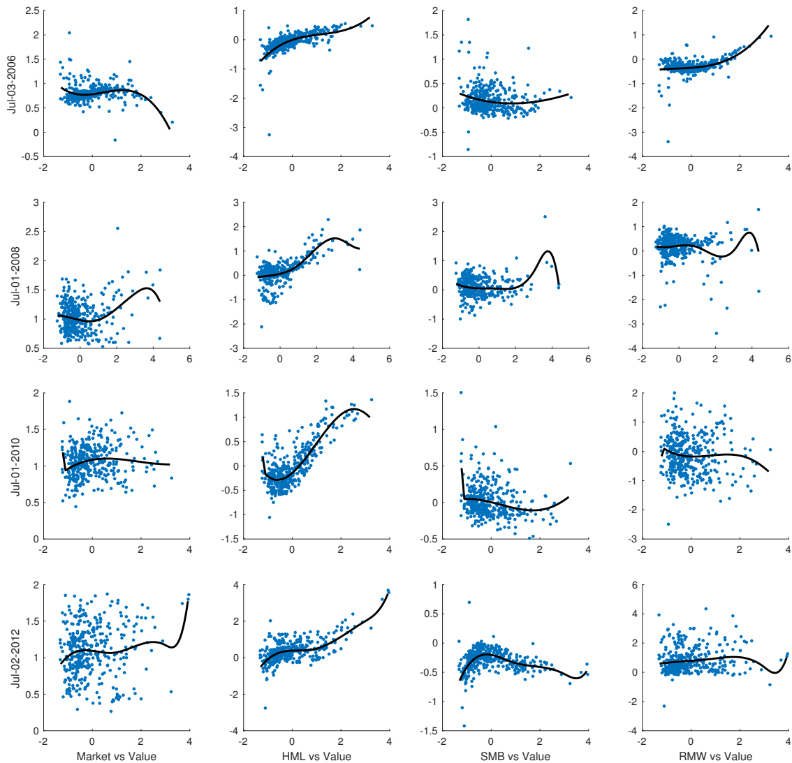
Figure 5: Different factors' G versus value at representative days
