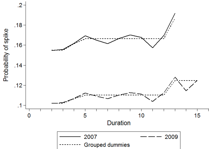
Figure 3.1: Baseline hazard
