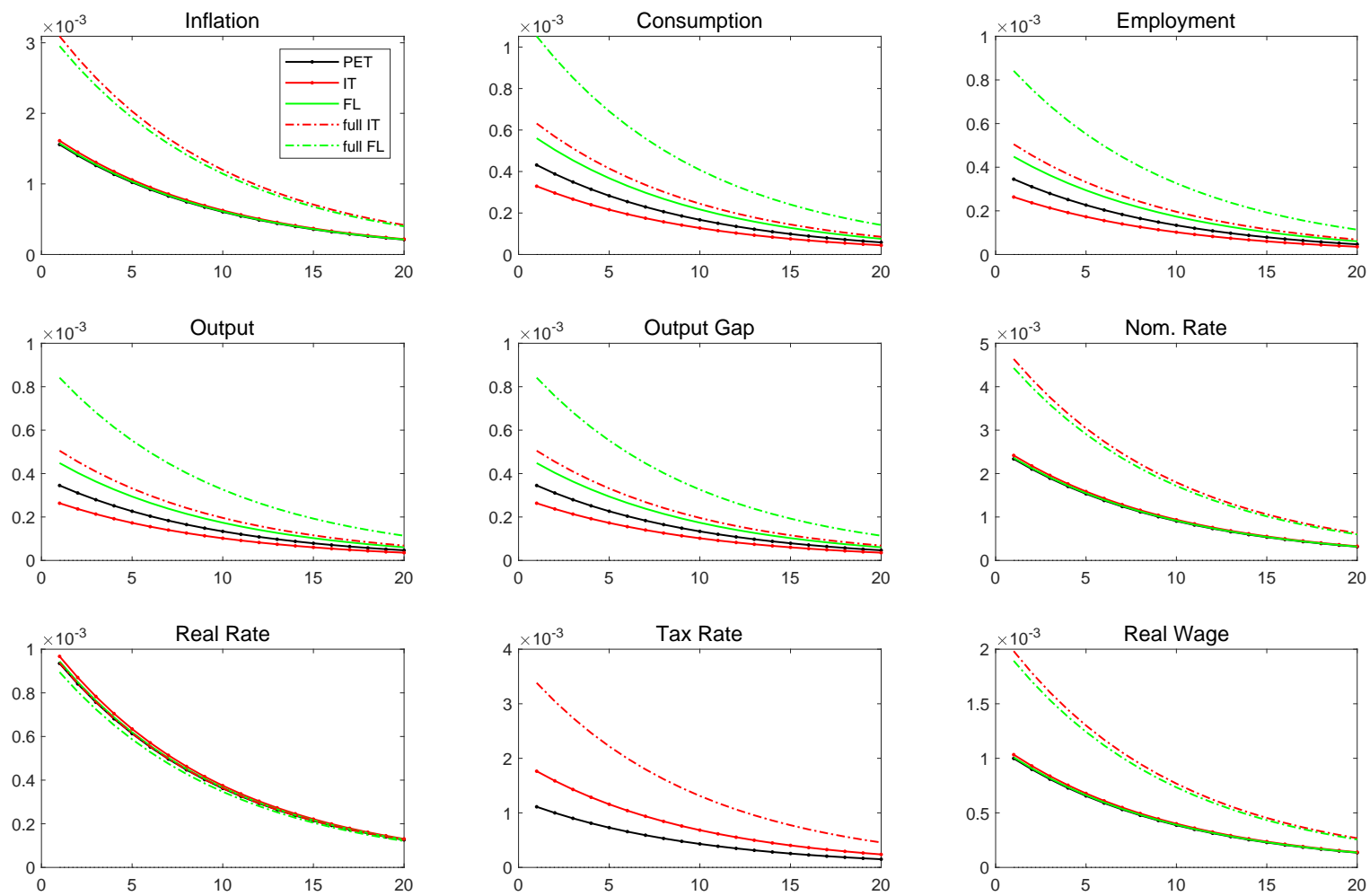
Figure 4: Impulse Responses to a Positive Time Preference Shock
