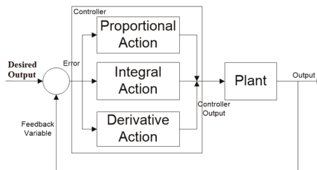
Figure 2. Proportional Integral Derivative (PID) controller.
