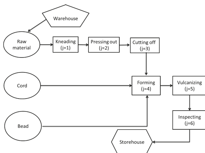
Figure 2. Tire manufacturing flow chart.
