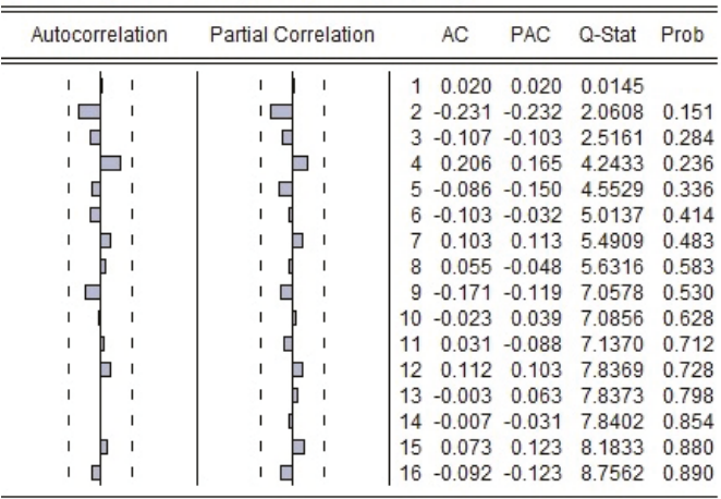
Figure 2. The correlogram of the residual error of the LS-ARIMAX i (2, 1, 1, X_{t-i} )-ECM model.
