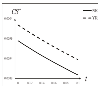
Figure 5. The optimal CS^* with respect to t .
