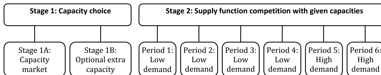
Figure 3: Timing of a round in CAPMARKET.
